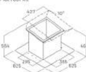
Kit techo plano Flat roof kit
